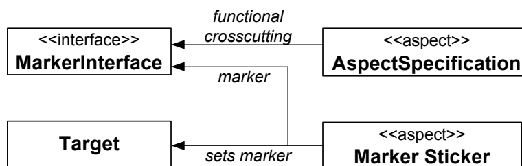
Figure 4. Marker Interface, Aspect Specification and Marker Setter
