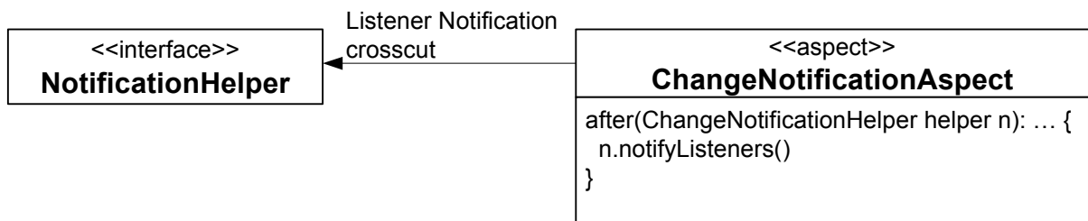
Figure 13. Marker Interface application
