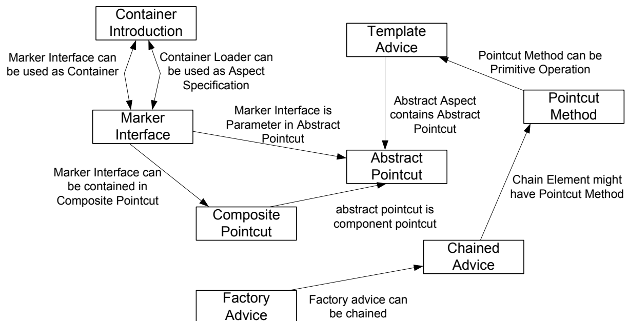
Figure 2. AspectJ idioms and their relationship to each other
