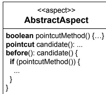
Figure 8. POINTCUT METHOD with Candidate Pointcut and Conditional Advice
