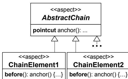
Figure 9. CHAINED ADVICE with Anchor Pointcut inside the Abstract Chain and Chain Elements , each defining its own Chained Advice referring the Anchor Pointcut .
