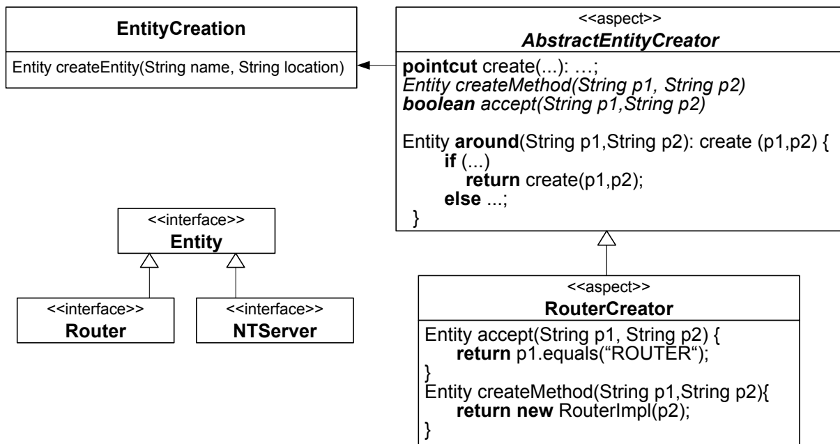
Figure 11. Implementation of ADVICED CREATIONAL METHOD based on POINTCUT METHOD and TEMPLATE ADVICE
