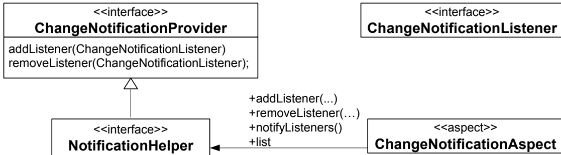
Figure 12. Applied Container Introduction
