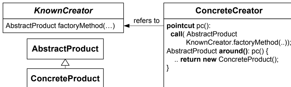
Figure 10. ADVISED CREATION METHOD
