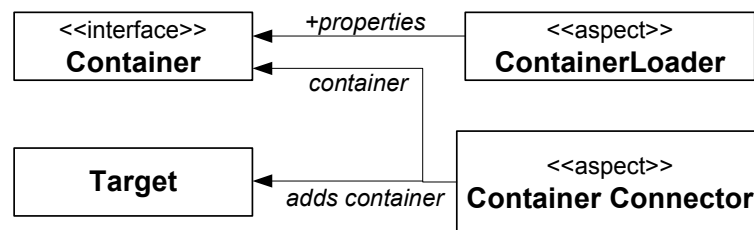
Figure 3. Container, Container Loader, Container Connector and Target Class in a CONTAINER INTRODUCTION
