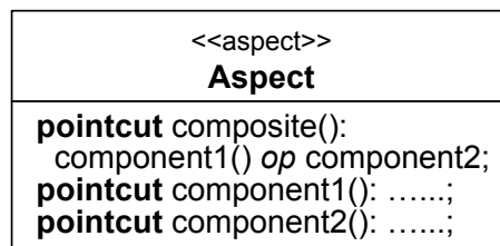
Figure 6. Composite Pointcut and corresponding Component Pointcuts
