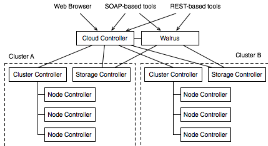
Figure 4: Eucalyptus' main components
