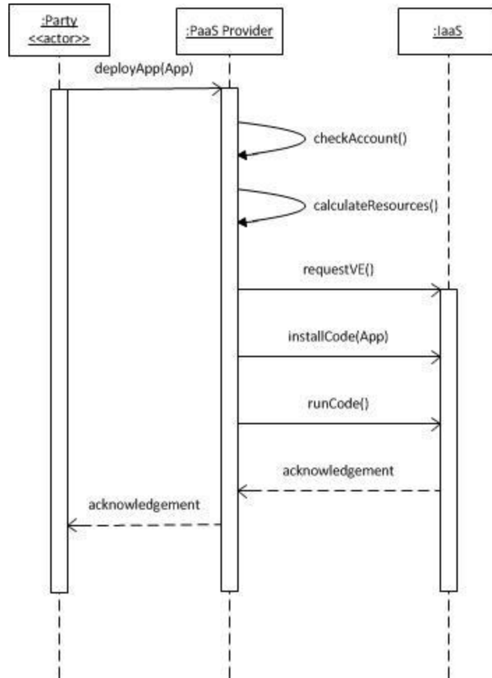
Figure 7: Sequence Diagram for Deploying an Application
