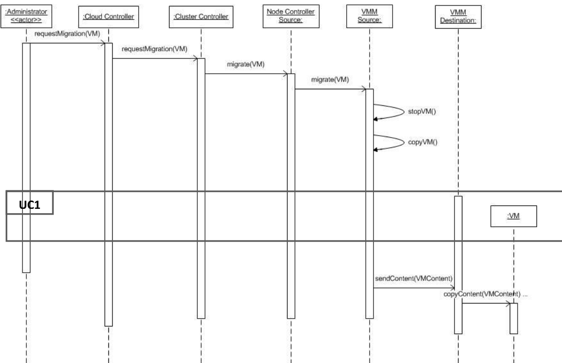
Figure 3: Sequence Diagram for Use Case Migrate a Virtual Machine
