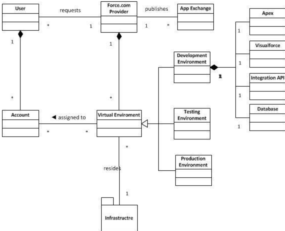
Figure 10: Class Diagram of Force.com's PaaS architecture
