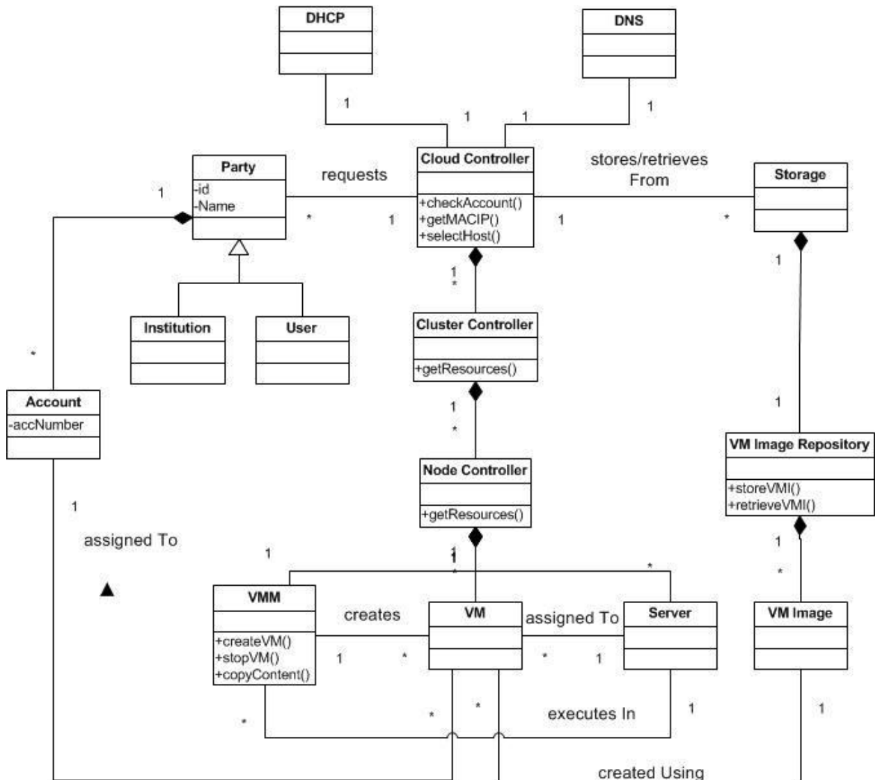
Figure 1: Class Diagram for a Cloud Infrastructure
