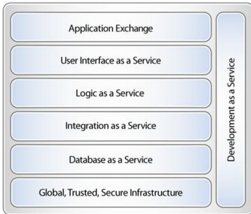
Figure 9: The Force.com stack and services (from [Sal2])
