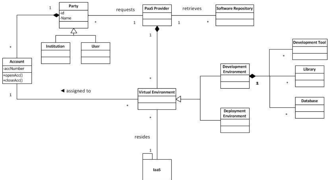
Figure 5: Class Diagram for PaaS Pattern
