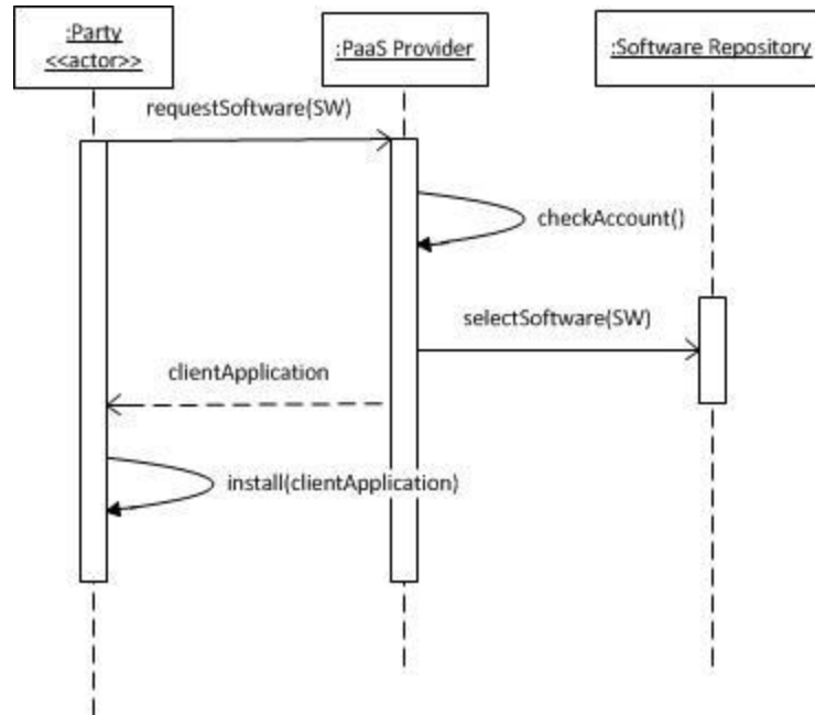
Figure 6: Sequence Diagram for Consuming Development Software
