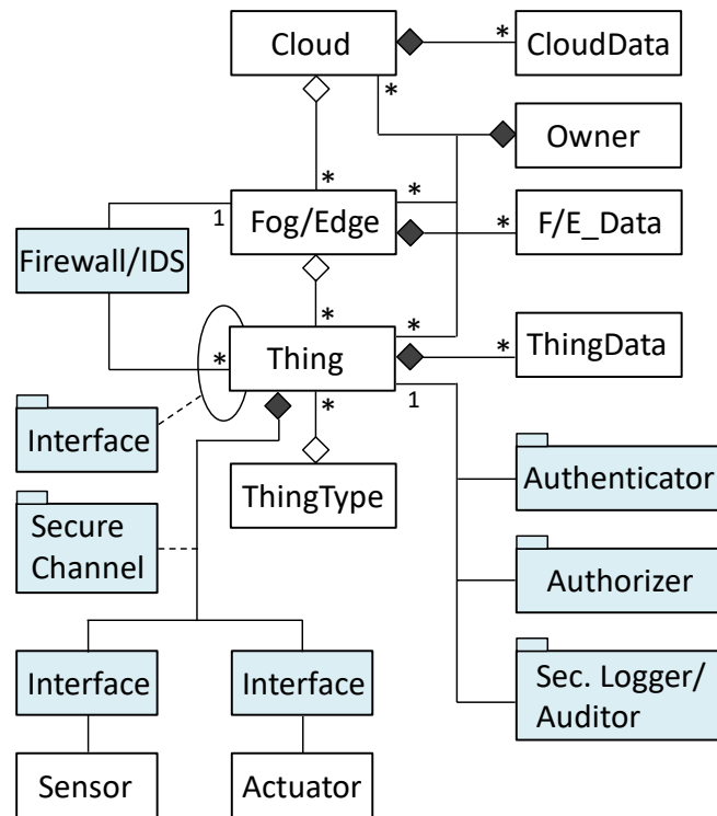
Fig. 4. A secure IoT architecture
