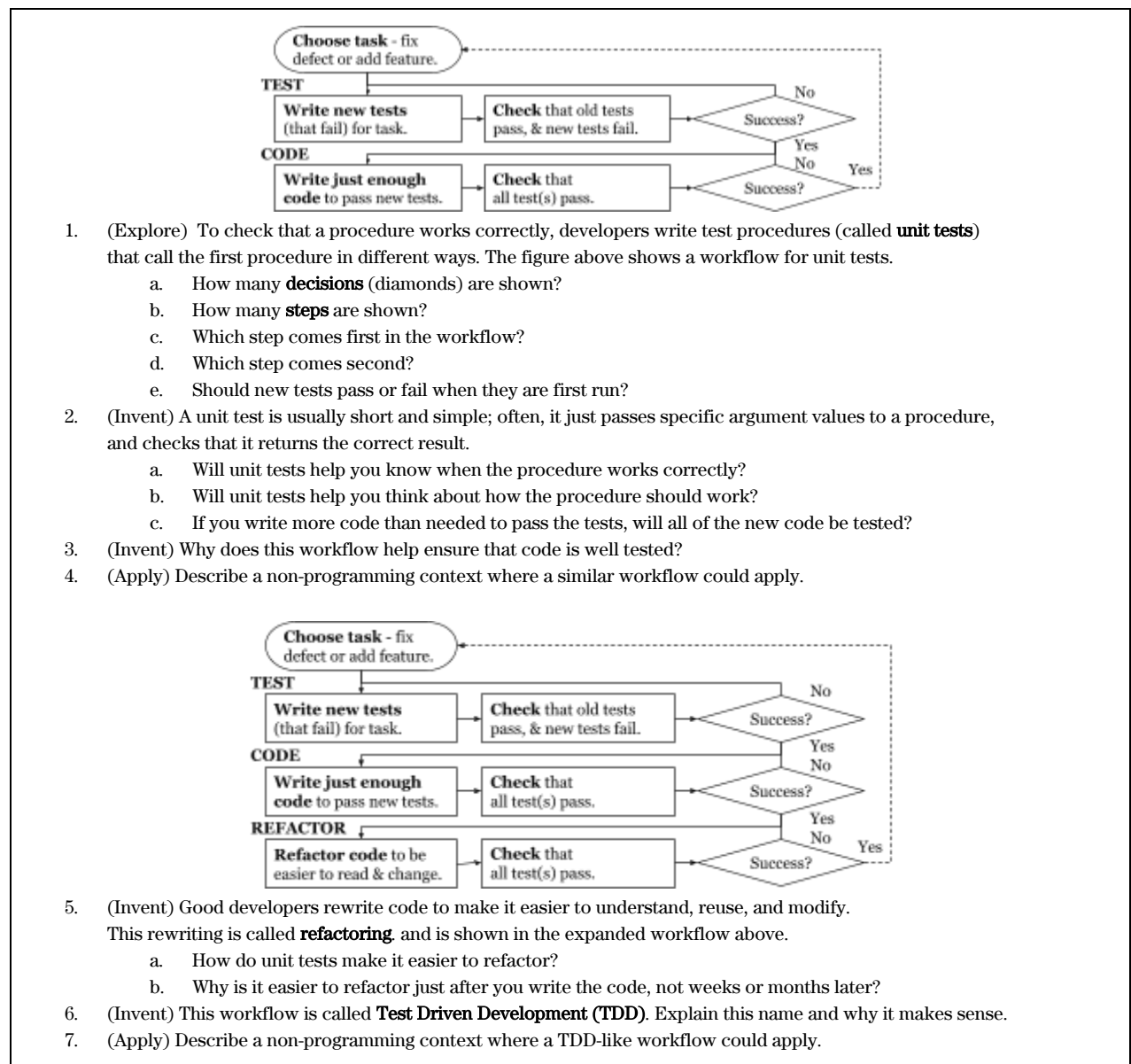
Figure 5: Sample MODEL: DIAGRAM with EIA LEARNING CYCLE Questions for Flowcharts
