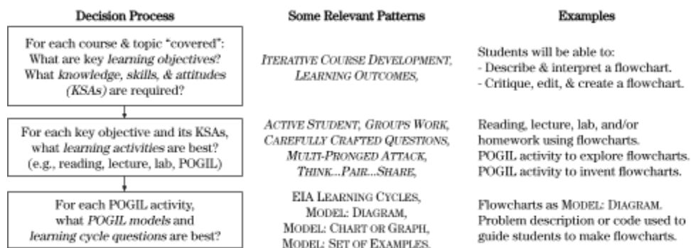
Figure 1: Using patterns at multiple levels to plan learning activities.
