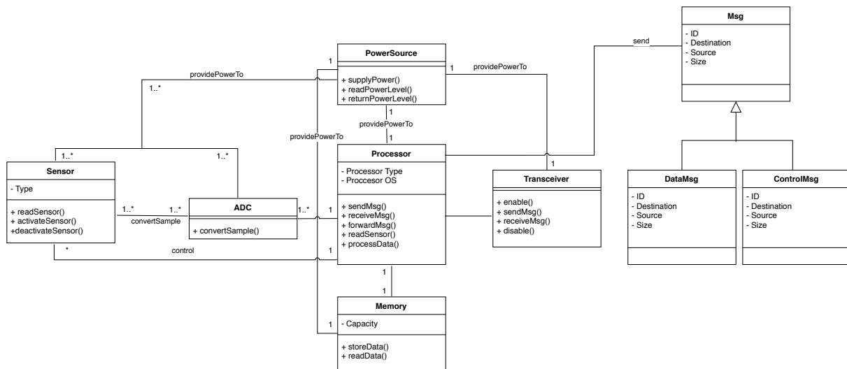
Fig. 2. Class diagram of the Sensor Node
