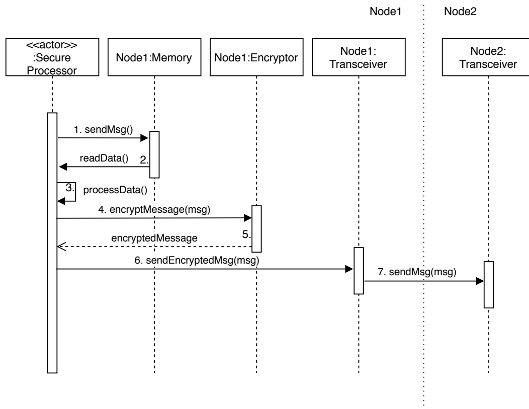
Fig. 4. Sequence diagram of use case "Send encrypted message from Node1 to Node2"
