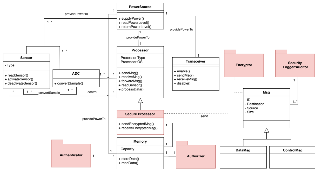
Fig. 3. Class diagram of Secure Sensor Node
